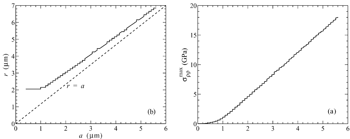
Fig. 4. (a) Evolution of the maximum radial stress at the coating surface \sigma_{\rho\rho}^{\max} with the contact radius a and (b) the corresponding location r at the coating surface at which the stress is maximum.
