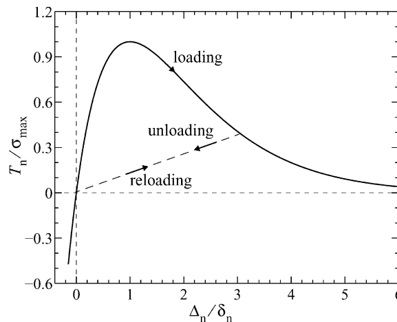
Fig. 11. Irreversible normal cohesive traction T_n(\Delta_n) at \Delta_t = 0 .
